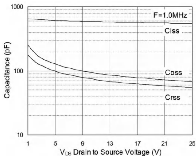
Fig.7 Capacitance
