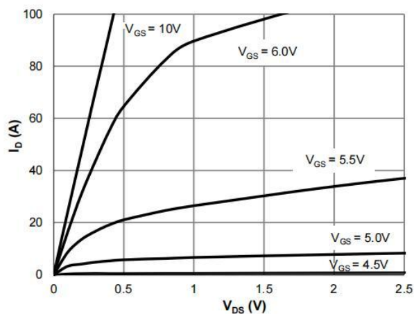
Figure 1: Saturation Characteristics
