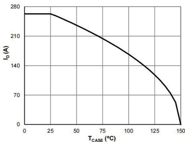
Figure 9: Current De-rating
