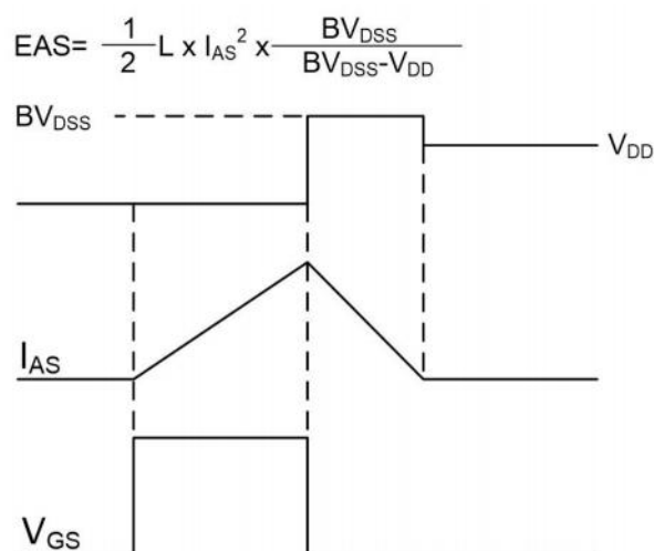
Fig.11 Unclamped Inductive Switching Waveform
