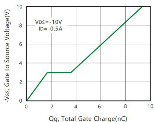
Figure 6. Gate Charge
