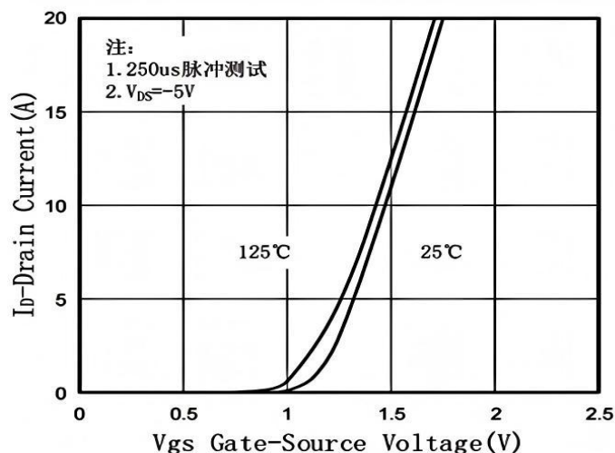
Fig.3 Transfer Characteristic
