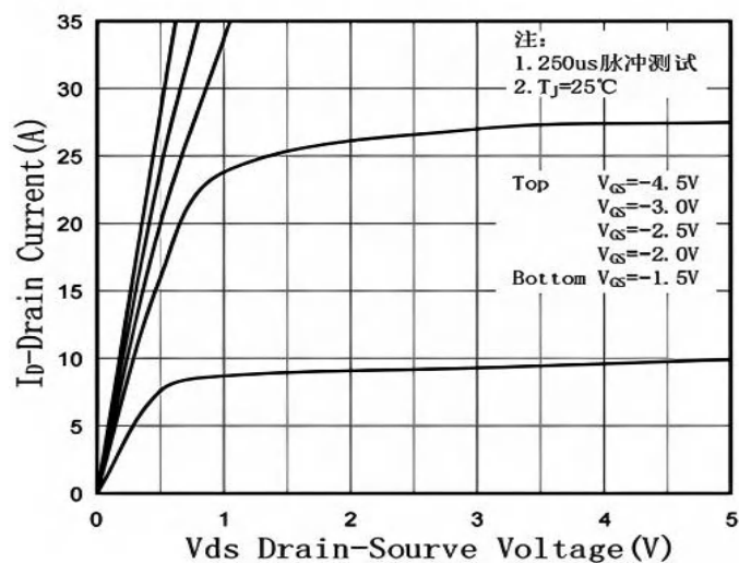
Fig.1 Output Characteristic
