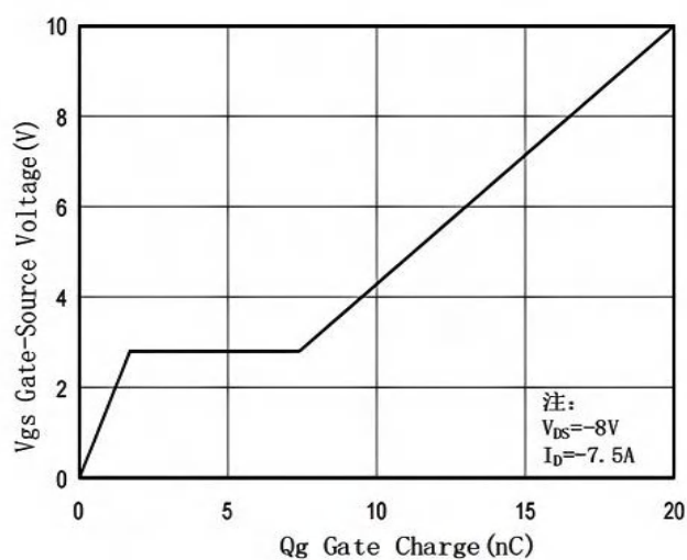
Fig.7 Gate-Charge Characteristic
