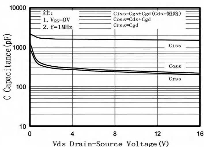
Fig.6 Capacitance Characteristic
