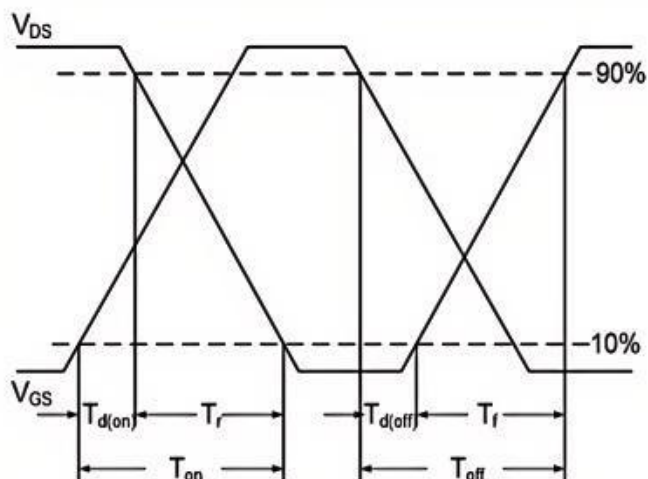
Fig.9 Switching Time Waveform
