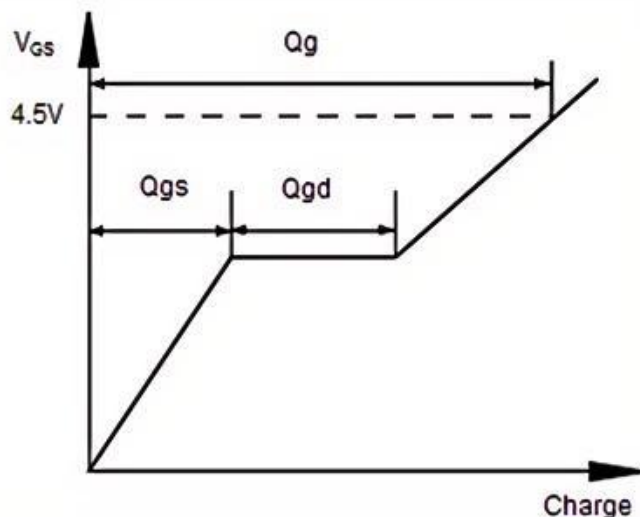
Fig.10 Gate Charge Waveform
