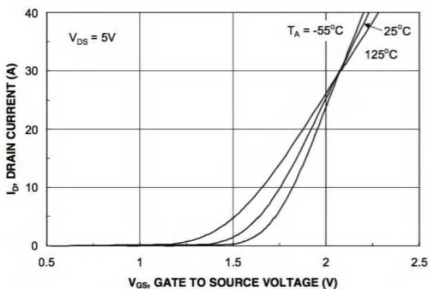
Figure 5. Transfer Characteristics.
