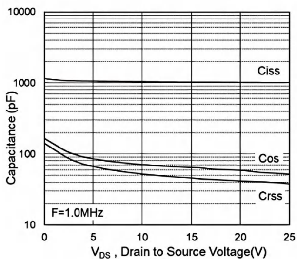
Fig.7 Capacitance
