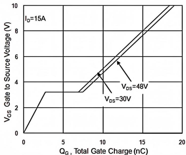
Fig.4 Gate-Charge Characteristics
