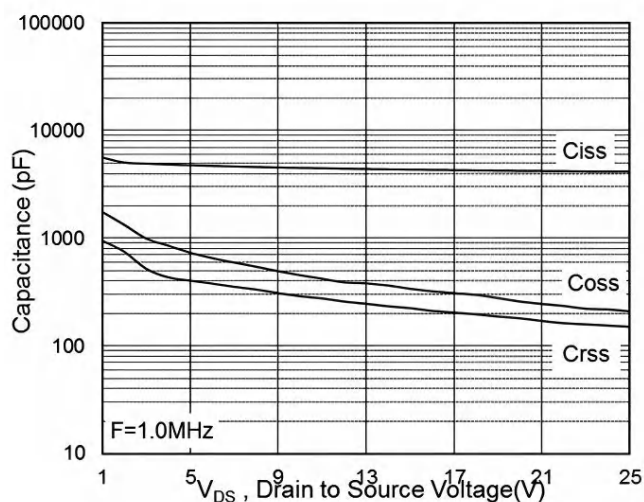
Fig.7 Capacitance
