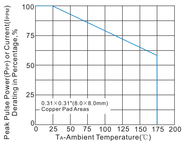
Fig.1 Power Derating Cure
