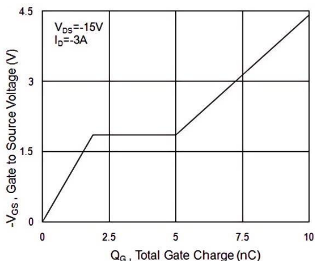
Fig.4 Gate-Charge Characteristics
