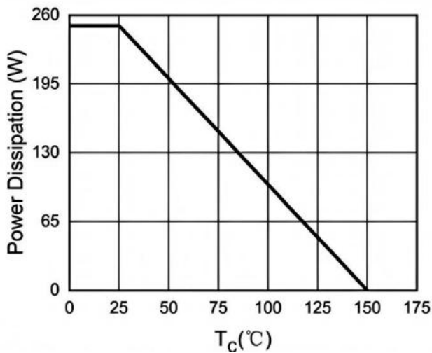
Fig.3 Power Dissipation
