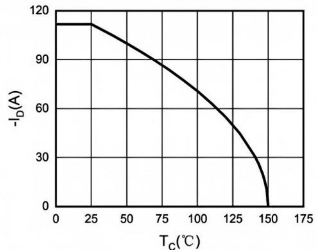
Fig.4 Drain Current
