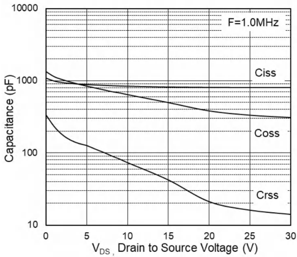
Fig.7 Capacitance
