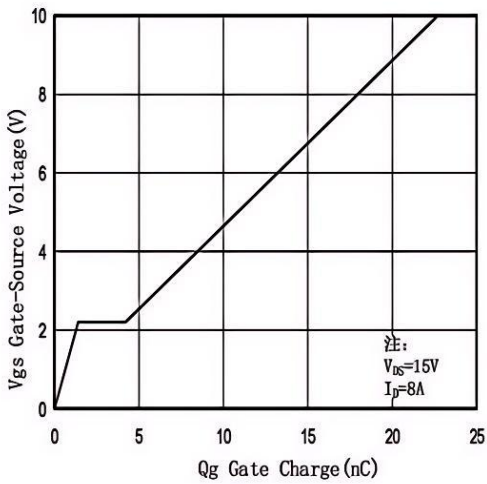
Fig.7 Gate-Charge Characteristic
