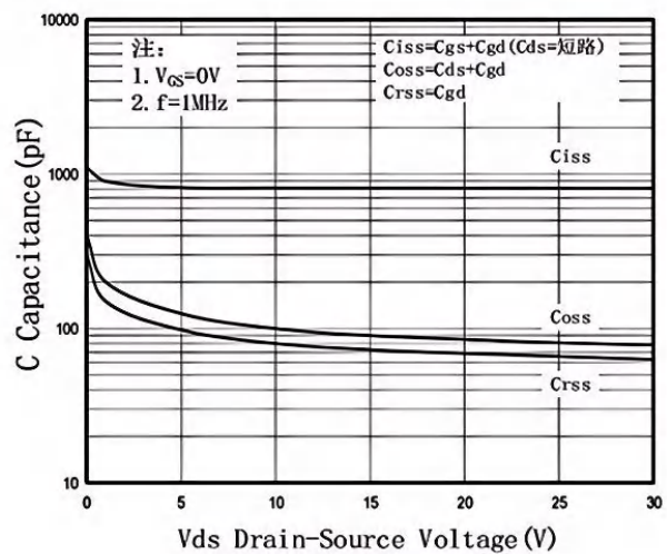
Fig.6 Capacitance Characteristic
