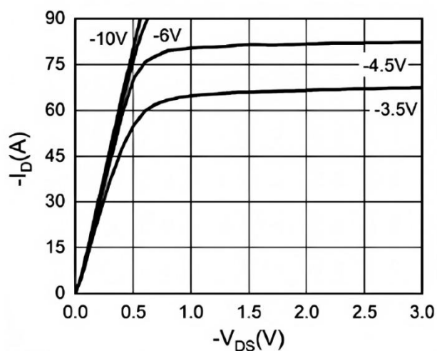
Fig.1 Output Characteristics
