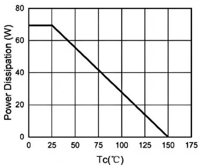
Fig.3 Power Dissipation
