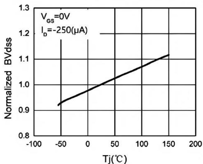
Fig.5 BV_{DSS} vs Junction Temperature
