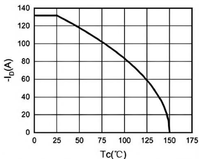
Fig.4 Drain Current
