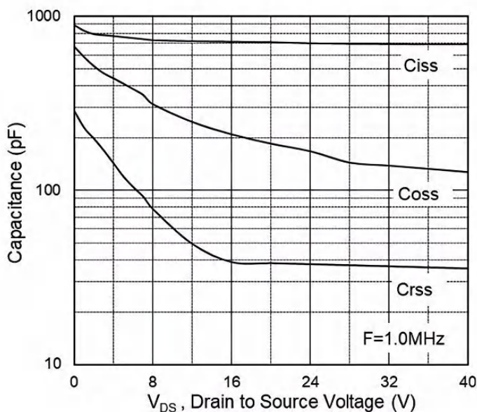
Fig.7 Capacitance
