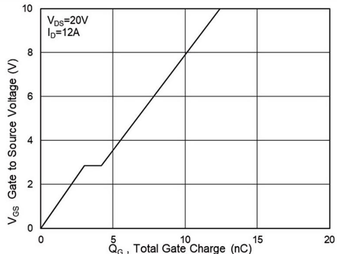
Fig.4 Gate-Charge Characteristics
