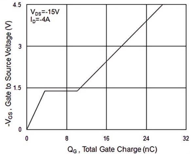
Fig.4 Gate-Charge Characteristics
