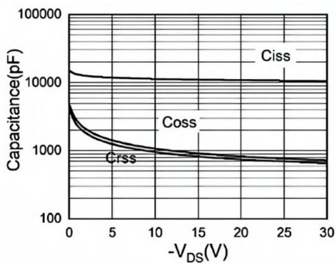
Fig.8 Capacitance
