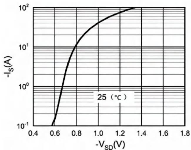
Fig.9 Body-Diode Characteristics
