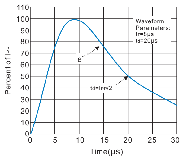
Fig. 2 Pulse Waveform
