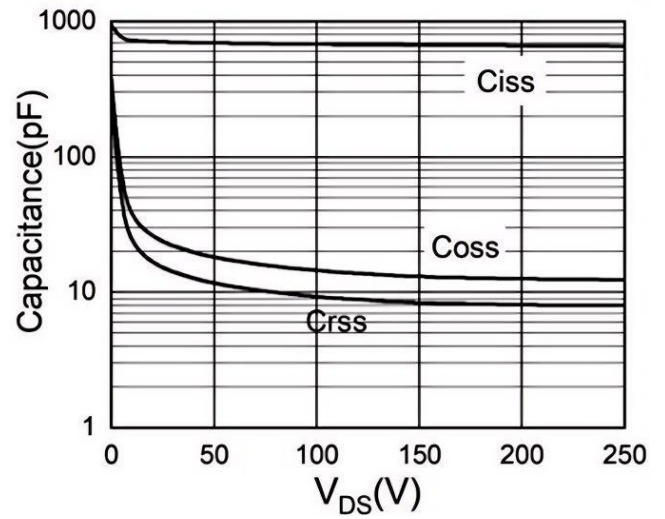
Fig.8 Capacitance
