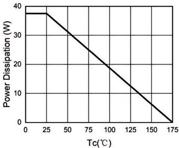
Fig.3 Power Dissipation
