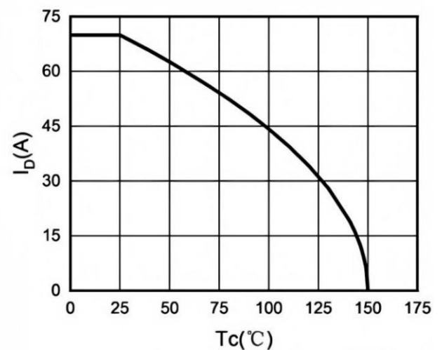
Fig.4 Drain Current
