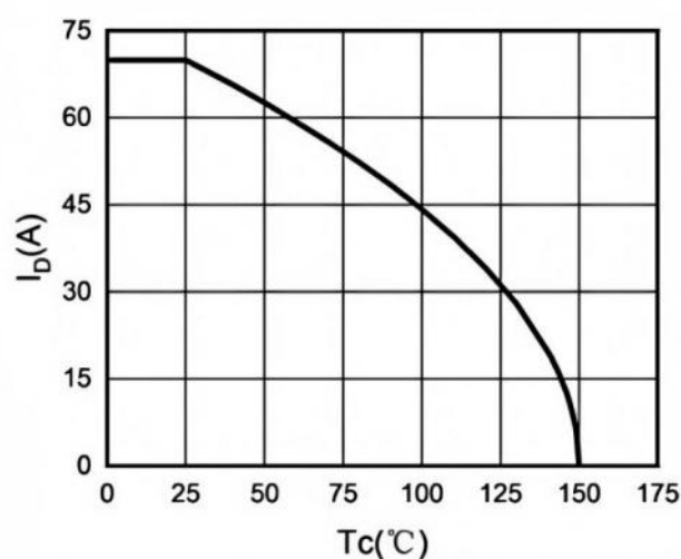
Fig.4 Drain Current
