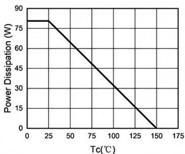
Fig.3 Power Dissipation
