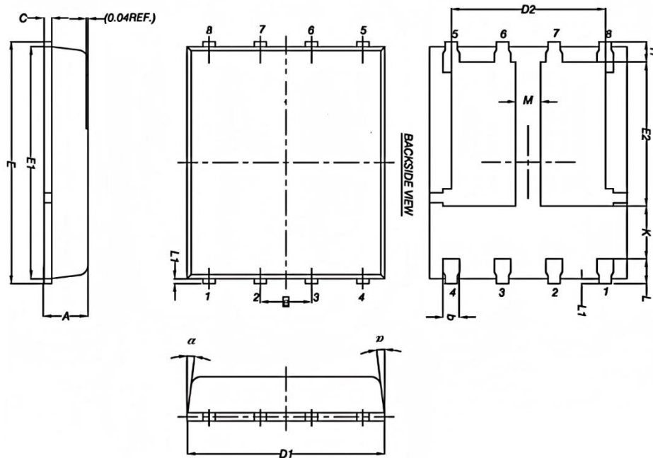
PRPAK5*6 Package Outline
