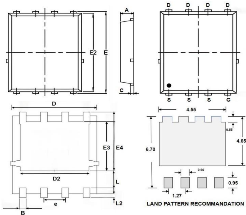
PRPAK5*6 Outline
