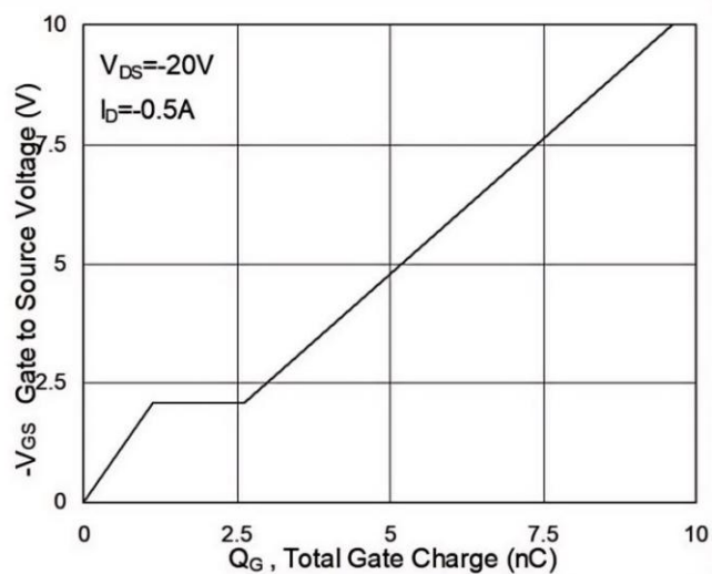
Fig.2 Gate-Charge Characteristics
