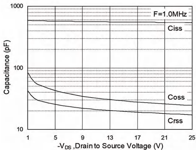
Fig.5 Capacitance
