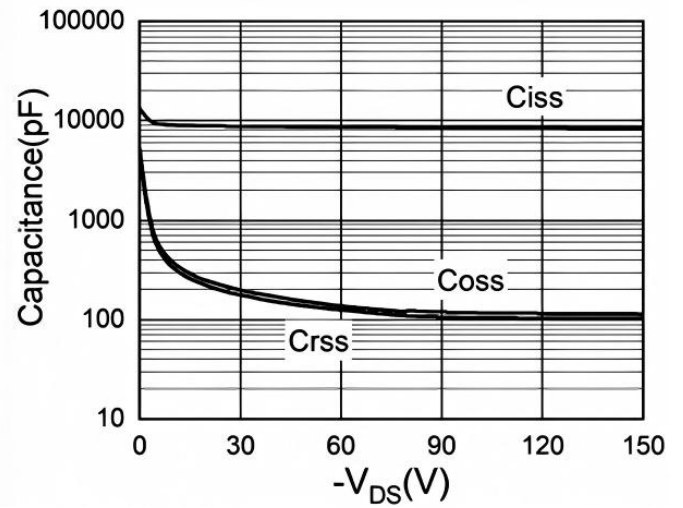
Fig.8 Capacitance
