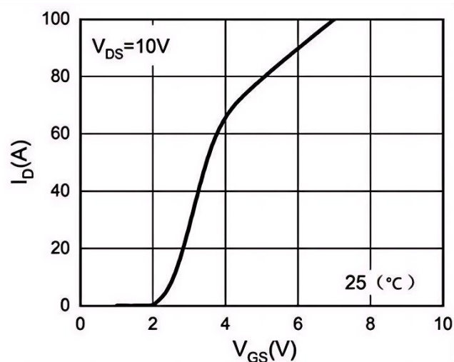
Fig.2 Transfer Characteristics
