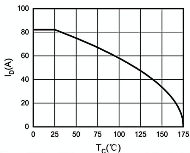
Fig.4 Drain Current
