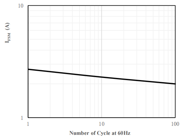
Fig 6 Surge Current Derating Curve
