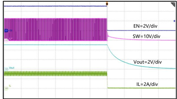
Figure 21. Shut-down with EN, I_{OUT}=3A
