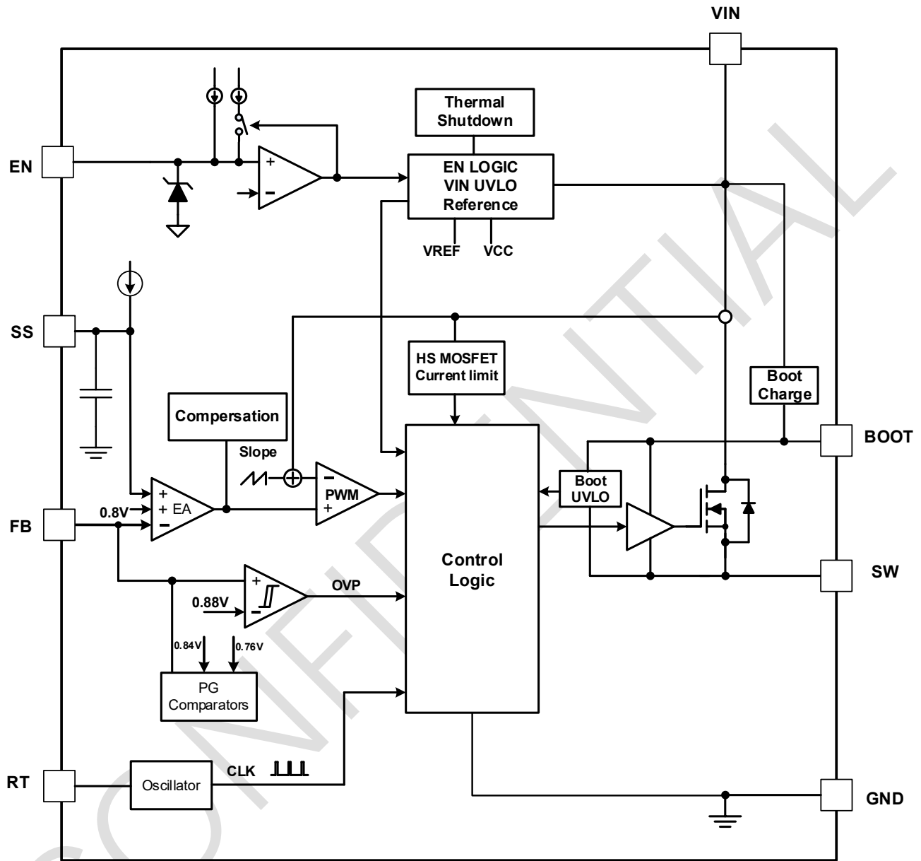
Figure 11. Block Diagram of GBI1630A
