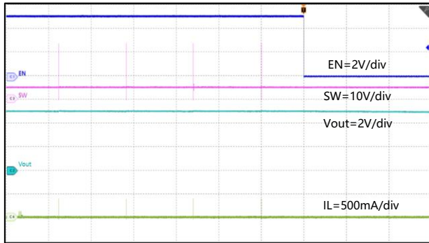
Figure 20. Shut-down with EN, I_{OUT}=0A
