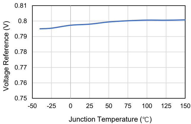
Figure 9. VREF Vs. Junction Temperature
