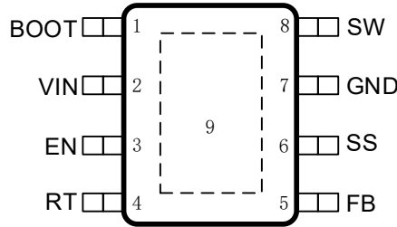
Top View: GBI1630A eSOP-8L
