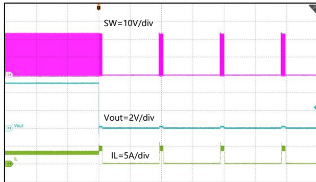
Figure 28. Normal Operation to Hard-short I_{OUT}=3A
