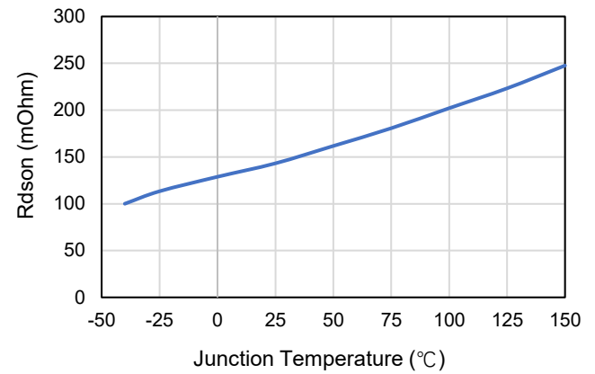
Figure 10. High Side MOSFET Rds(on)
