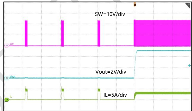
Figure 29. Hard-short Recovery I_{OUT}=3A
