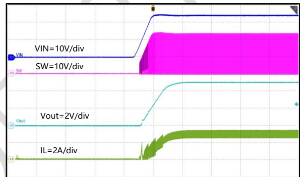
Figure 23. Start-Up with VIN Rising, I_{OUT}=3A
