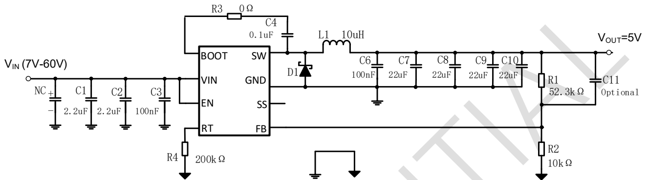
Figure 13. 24V Input Voltage, 5V/3A Output
