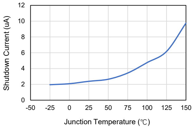
Figure 7. VIN Shutdown Current
