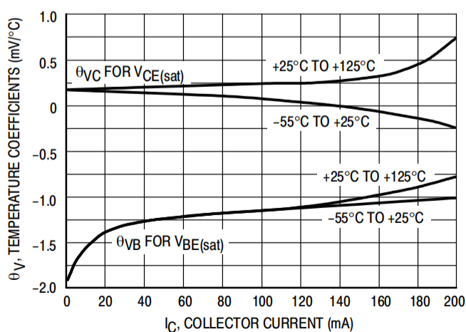
Figure 16. Temperature Coefficients
