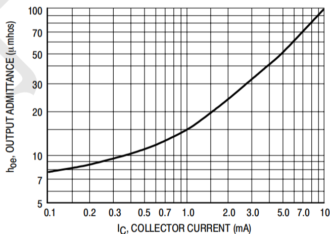
Figure 10. Output Admittance
