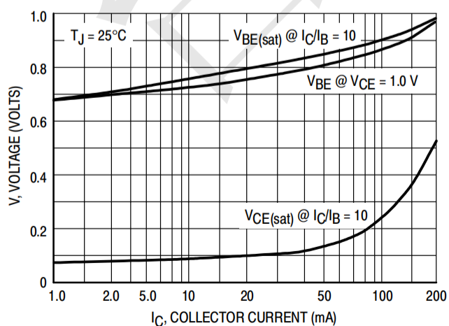
Figure 15. "ON" Voltages
