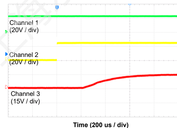
Figure 27. Power-Up with Enable
