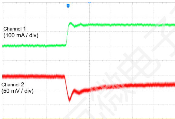
Figure 19. Load Transient (1 mA to 150 mA)
