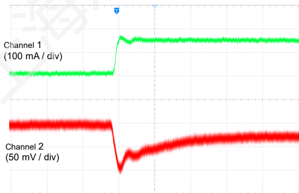
Figure 21. Load Transient (1 mA to 150 mA)
