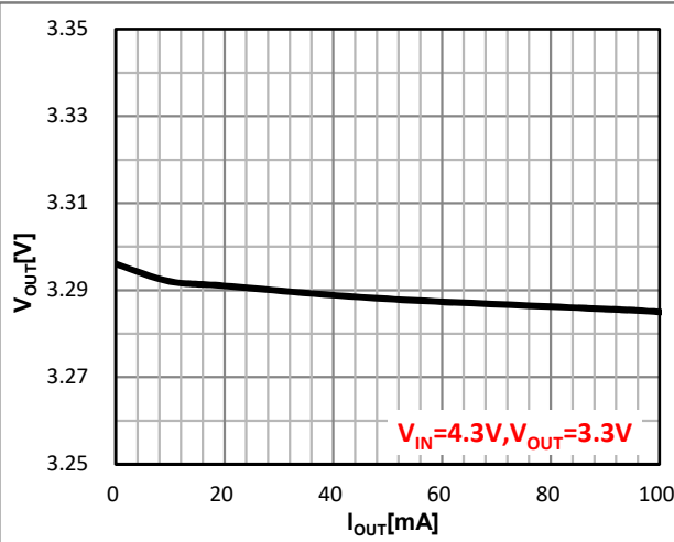
Figure 13. Load Regulation
