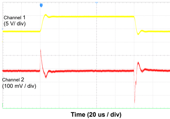
Figure 25. Line Transient
