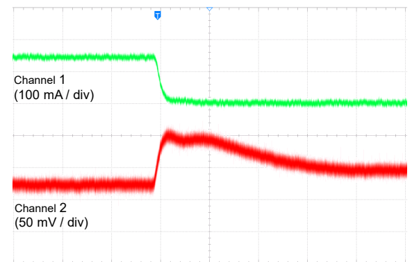
Figure 22. Load Transient (150 mA to 1 mA)
