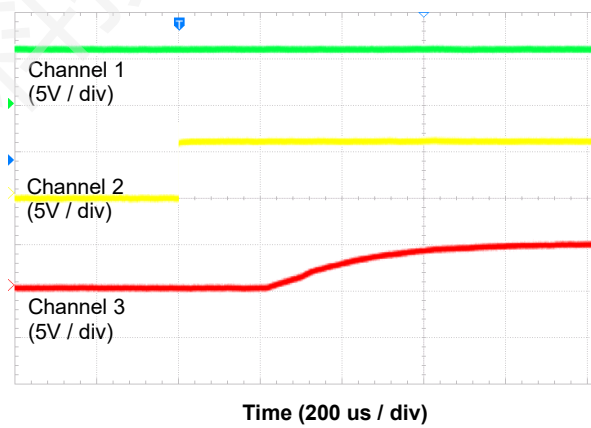
Figure 26. Line Transient
