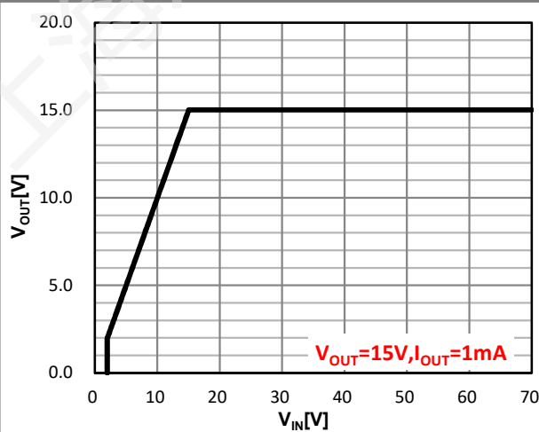
Figure 11. V_{OUT} vs V_{IN}
