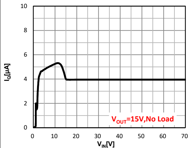
Figure 18. I_Q VS V_{IN}
