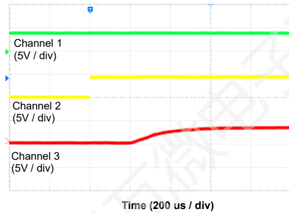
Figure 25. Line Transient
