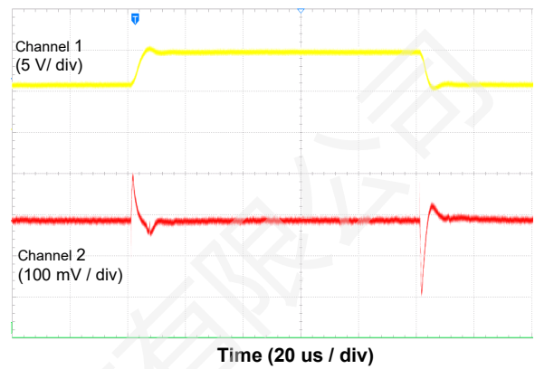
Figure 26. Line Transient
