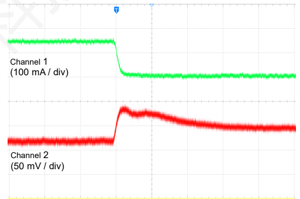
Figure 20. Load Transient (150 mA to 1 mA)
