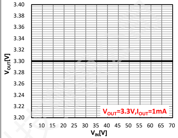
Figure 8. Line Regulation
