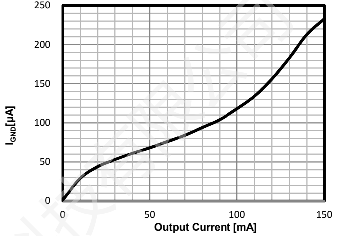
Figure 2. Ground Current vs Output Current
