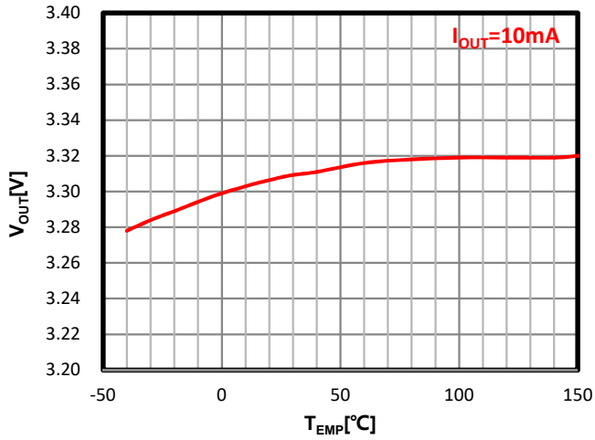
Figure 1. V_{OUT} vs Temperature
