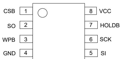
Figure 3-(a). Pin Configuration (SOP8*1, SOP-J8, TSSOP-B8, MSOP8) *1 Not Recommended for New Designs.
