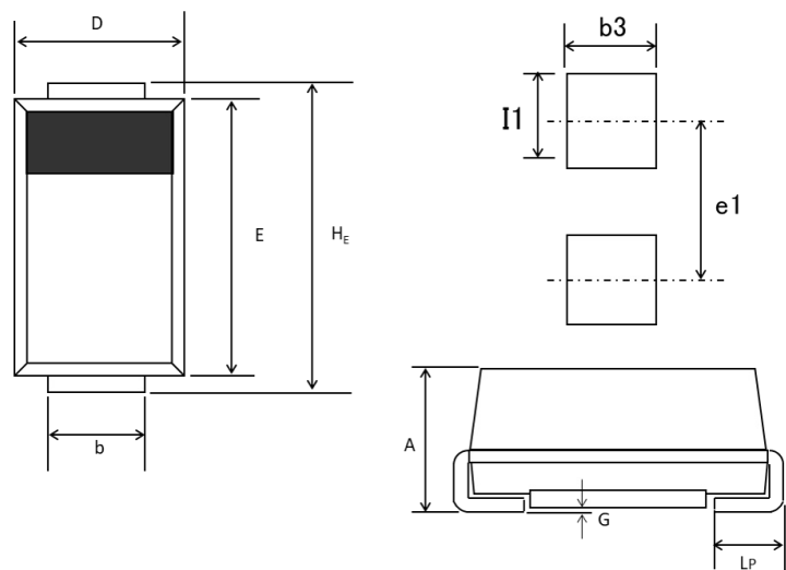
DO-214AC(SMA), (FMDS)
