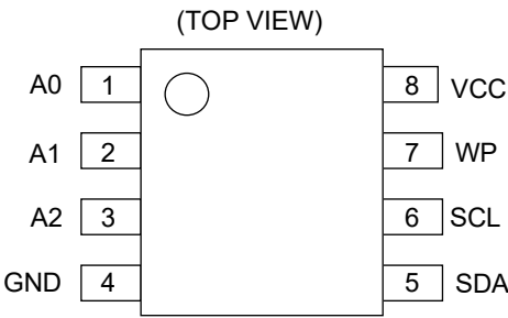
Figure 3-(a). Pin Configuration (SOP8*1, SOP-J8, TSSOP-B8, MSOP8) *1 Not Recommended for New Designs.
