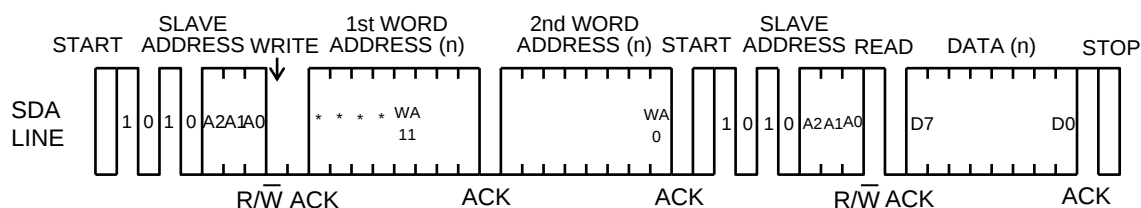
Figure 44. Random Read
