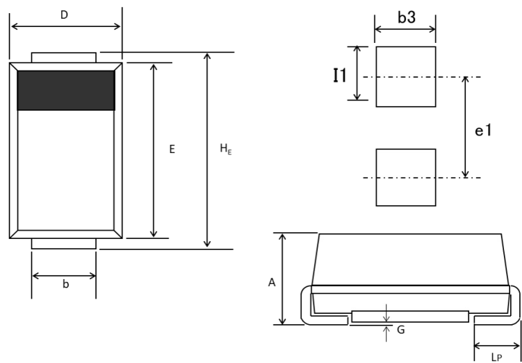
DO-214AC(SMA), (FVDS)
