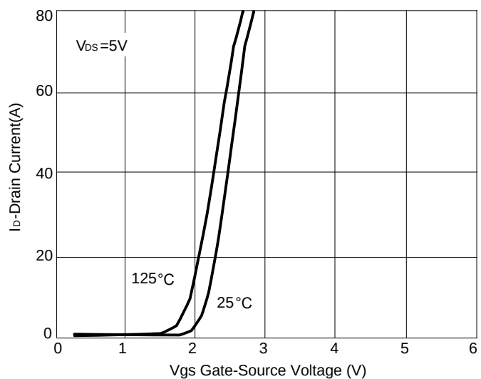
Figure 3: Transfer Characteristics
