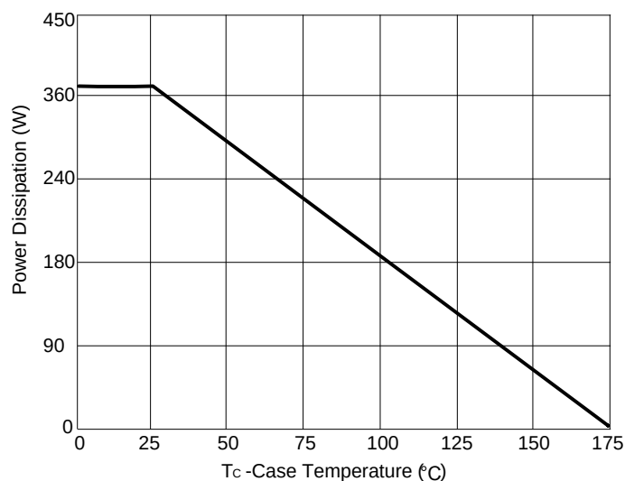
Figure 8: Power De-rating
