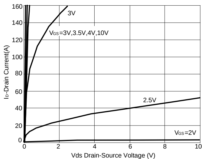
Figure 1: Output Characteristics
