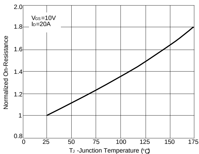
Figure 2: Rdson-Junction Temperature
