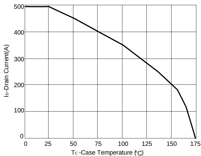
Figure 10: Current De-rating
