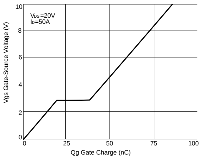
Figure 4: Gate Charge
