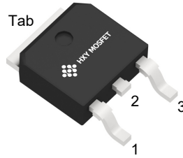
TO-252-2L
