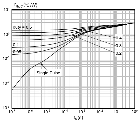
Figure 2. Maximum Transient Thermal Impedance
