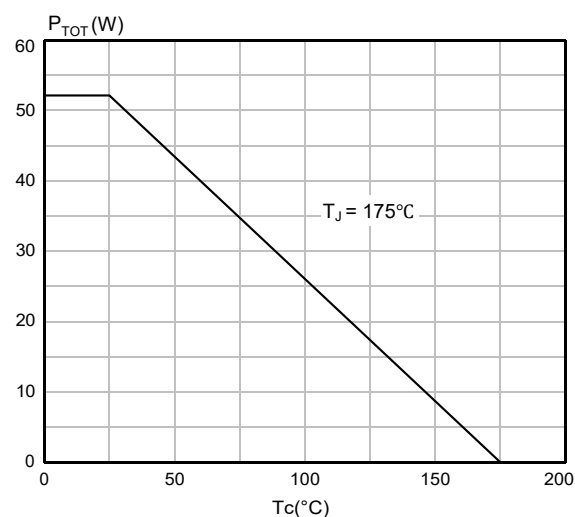
Figure 6. Total Power Dissipation
