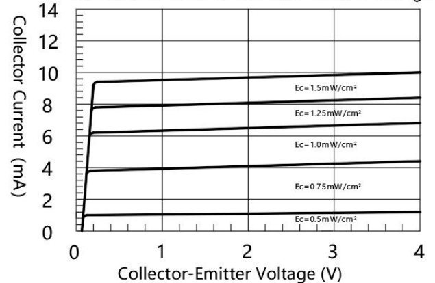
集电极电流与集电极-发射极电压关系 Collector Current VS Collector-Emitter Voltage
