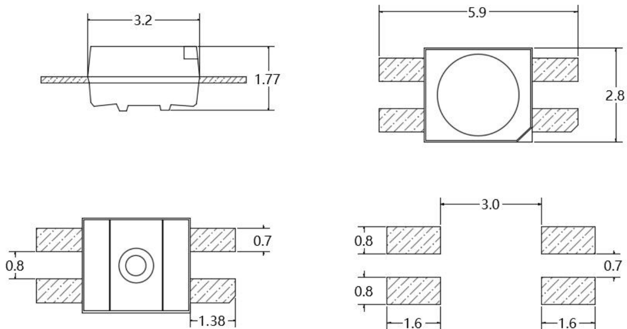
建议焊盘尺寸 Recommended Soldering Pattern
