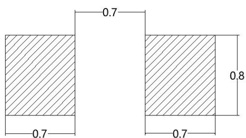
建议焊盘尺寸 Recommended Soldering Pattern
