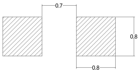
建议焊盘尺寸 Recommended Soldering Pattern
