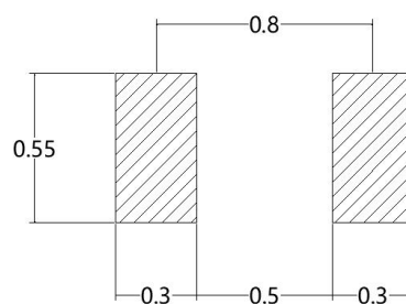
建议焊盘尺寸 Recommended Soldering Pattern
