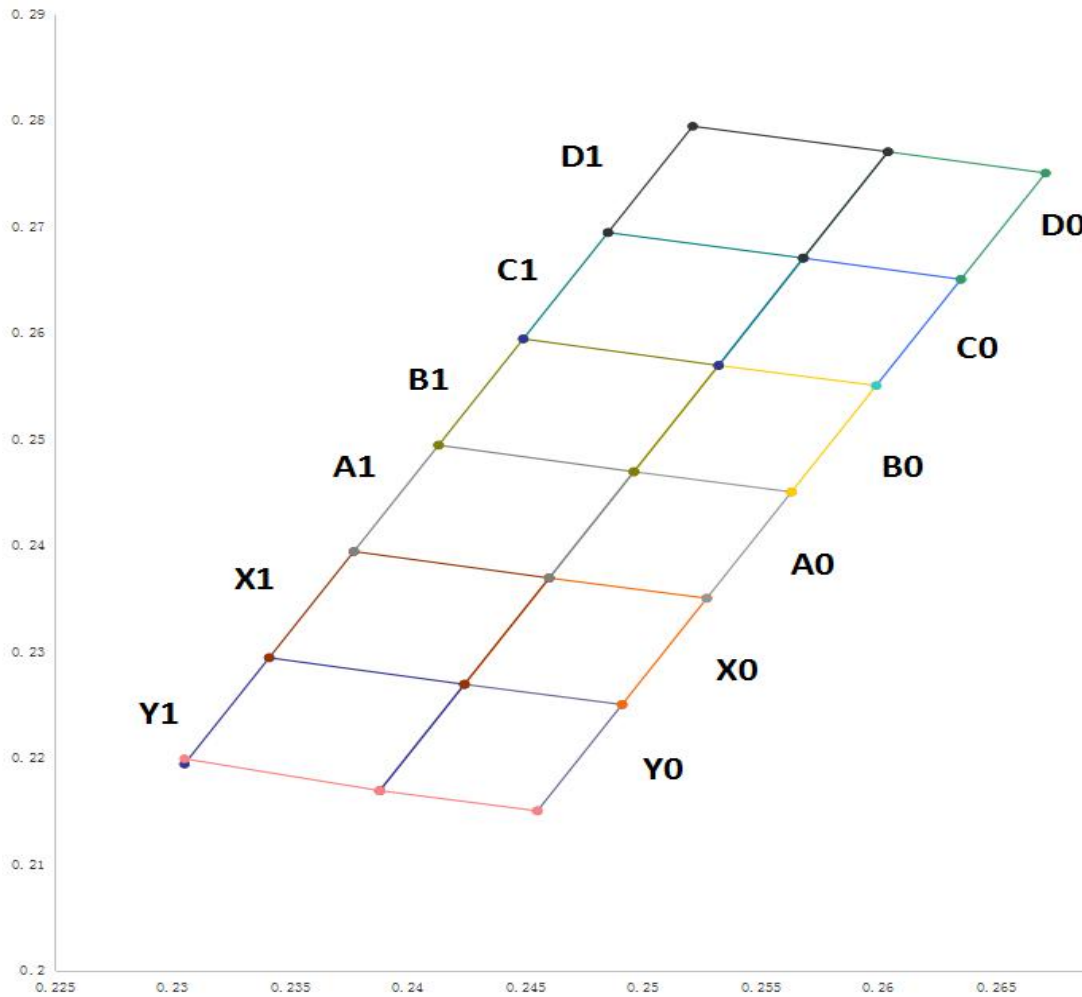
色度坐标范围 Bin Range of Chromaticity Coordinates
