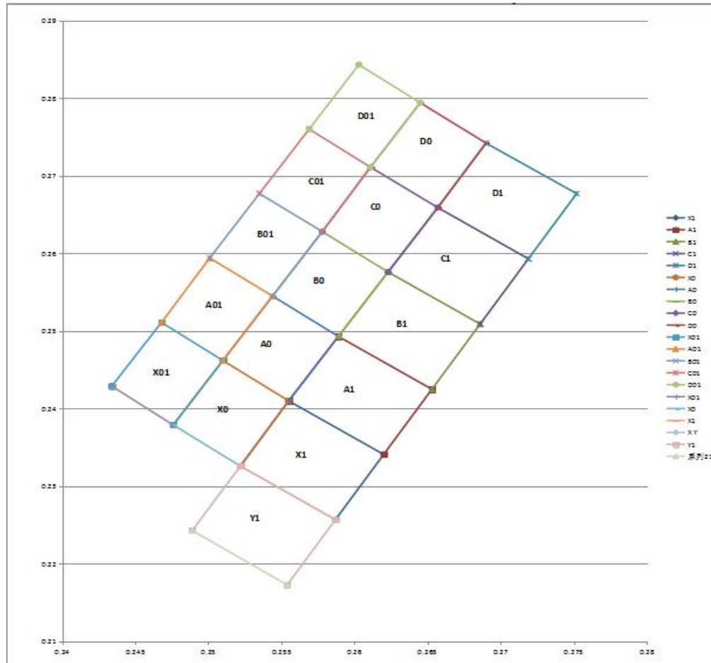
色度坐标范围 Bin Range of Chromaticity Coordinates
