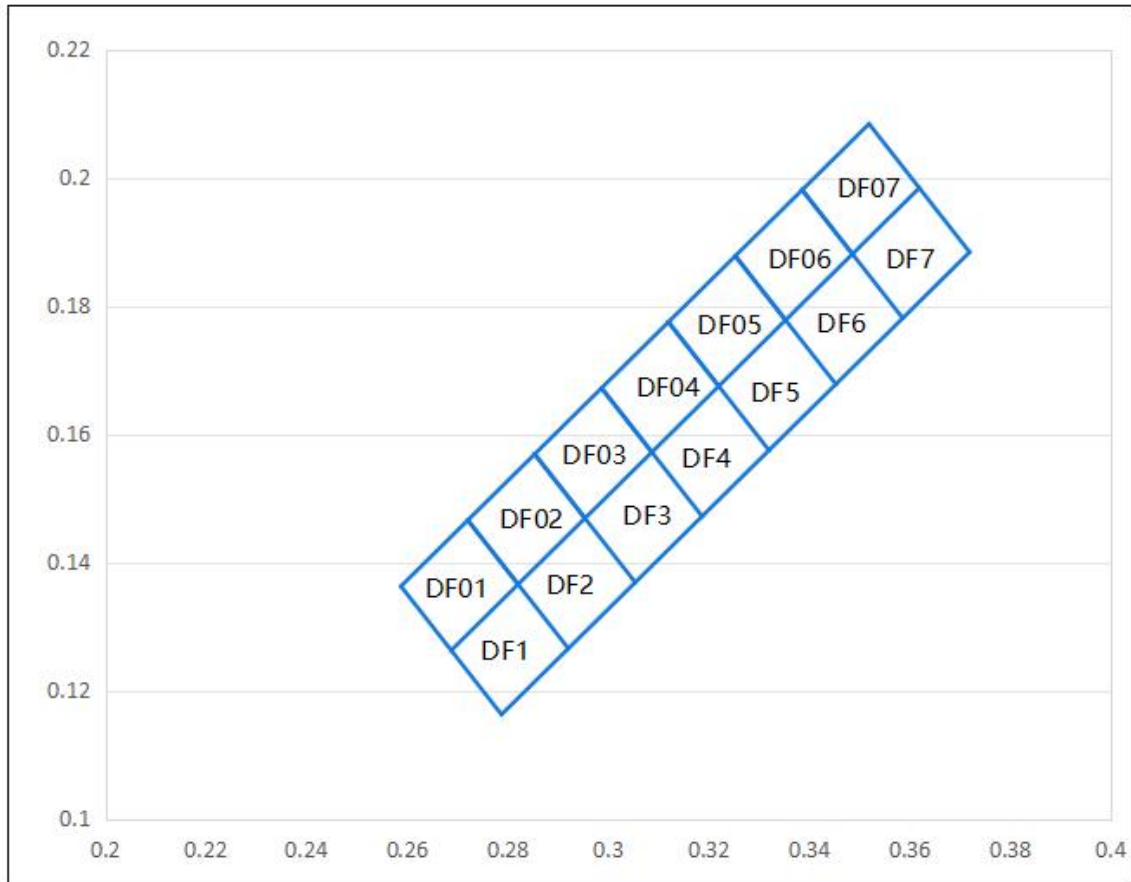
色度坐标范围 Bin Range of Chromaticity Coordinates
