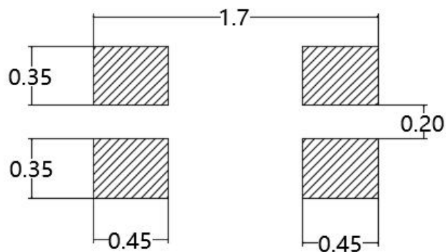
建议焊盘尺寸 Recommended Soldering Pattern
