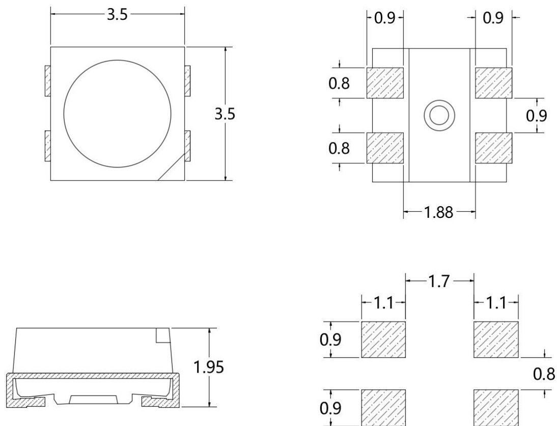
建议焊盘尺寸 Recommended Soldering Pattern
