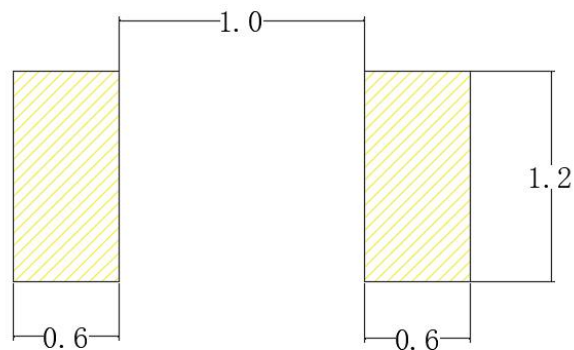
建议焊盘尺寸 Recommended Soldering Pattern
