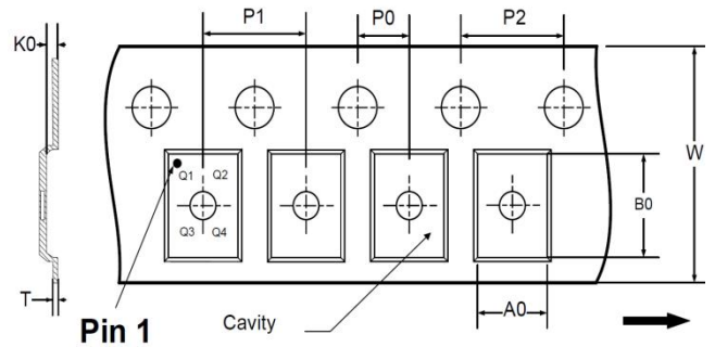
TAPE DIMENSIONS
