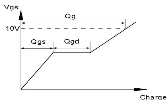
Figure 1 Gate Charge Test Circuit & Waveform
