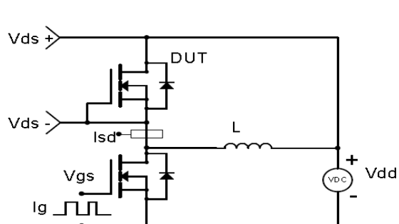
Figure 4 Diode Recovery Test Circuit & Waveforms www.doingter.cn
