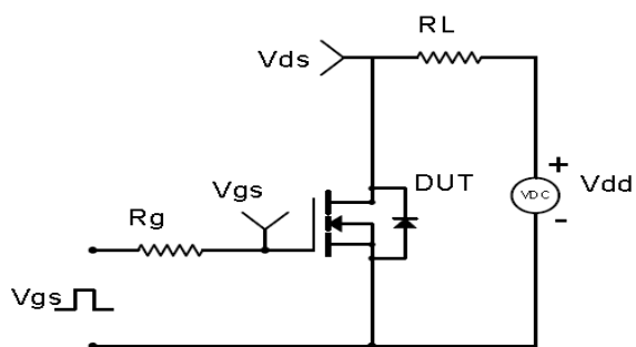
Figure 2 Resistive Switching Test Circuit & Waveforms
