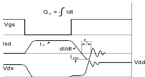
Figure 4 Diode Recovery Test Circuit & Waveforms www.doingter.cn
