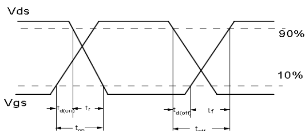
Figure 2 Resistive Switching Test Circuit & Waveforms
