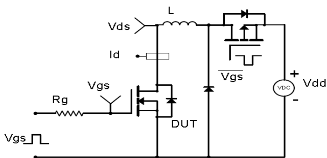
Figure 3 Unclamped Inductive Switching (UIS) Test Circuit & Waveforms
