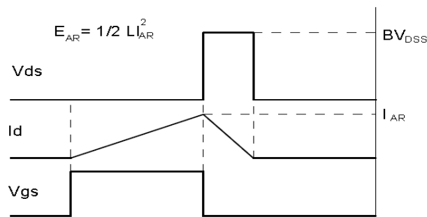
Figure 3 Unclamped Inductive Switching (UIS) Test Circuit & Waveforms
