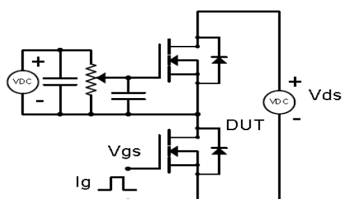
Figure 1 Gate Charge Test Circuit & Waveform
